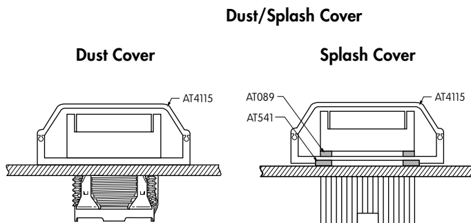
Snap-in Mount
