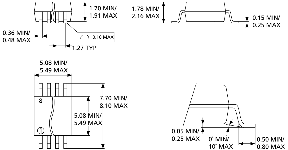
Figure 31: SO8W – 8 lead plastic small outline, 208 mils body width
