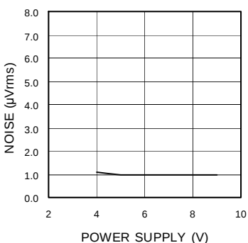
Fig.28 Output Noise Voltage (C,LS,RS,SW)- Power Supply Voltage (BD3818KS)
