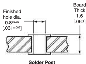
Solder Post
