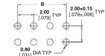
Recommended Solder Pad Layout
