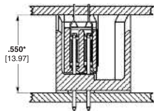
Figure 4 Double-Row, Two-Piece Receptacle and Two-Piece Shrouded Header *Mod II Shrouded Header Height is .440 [11.18] for a total stack height of .898 [22.80]
