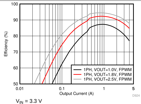
Figure 68. Efficiency in Forced-PWM Mode
