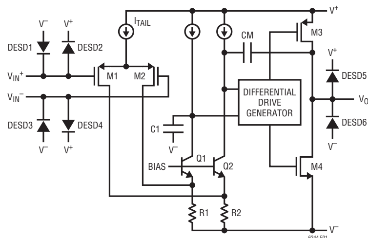
Figure 1. Simplified Schematic
