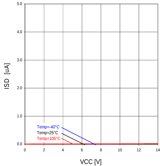
Fig.26 V_{CC}-I_{SD} ( V_{EN}=0V )
