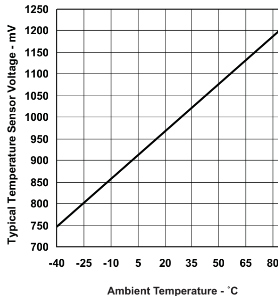
Figure 17. Typical Temperature Sensor Voltage
