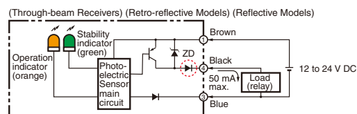
Models with PNP Output
