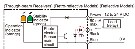
Models with NPN Output
