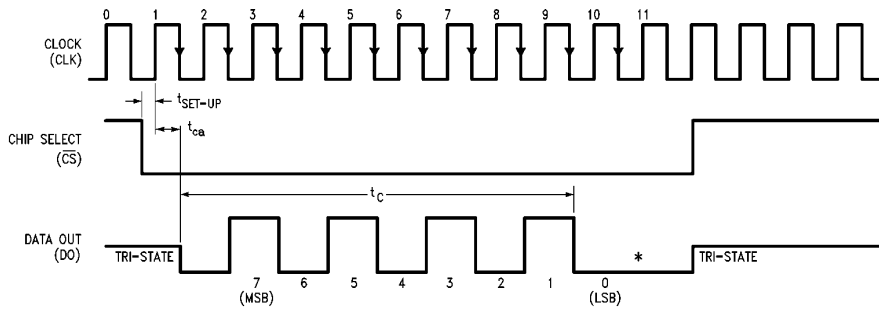
ADC08031 Timing
