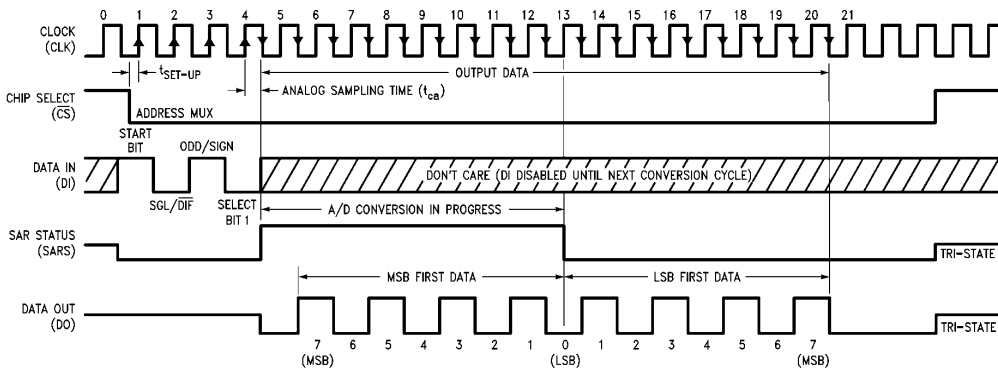
ADC08034 Timing
