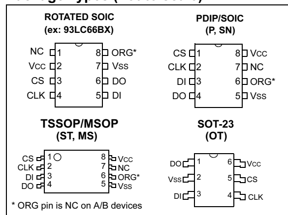
Package Types (not to scale)
