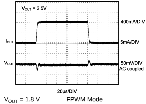
Figure 50. Load Transient Response
