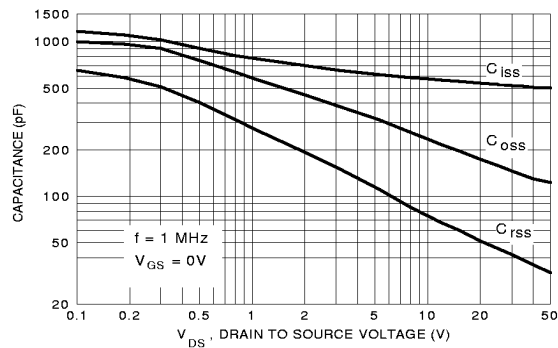
Figure 9. Capacitance Characteristics
