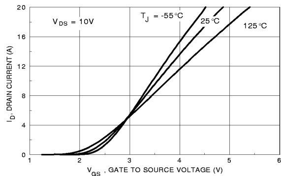
Figure 5. Transfer Characteristics
