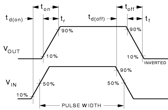
Figure 12. Switching Waveforms
