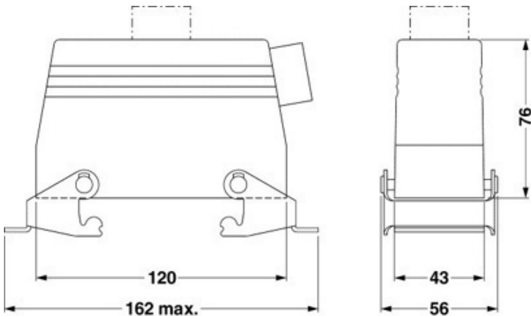
Dimensioned drawing
