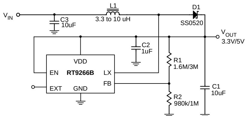
Figure 1. RT9266B Typical Application for Portable Instruments
