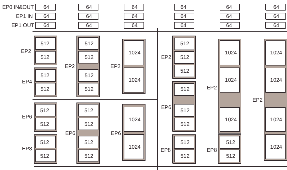
Figure 3-3. Endpoint Configuration
