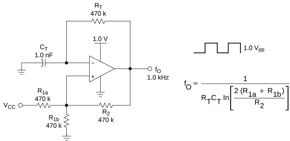
Figure 33. 1.0 V Oscillator
