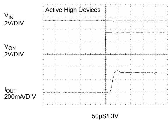
Figure 19. Current Limit Response Time (Output Shorted to GND by 10 \Omega , moderate short)
