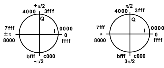
FIGURE 28. PHASE BIT MAPPING OF COORDINATE CONVERTER OUTPUT
