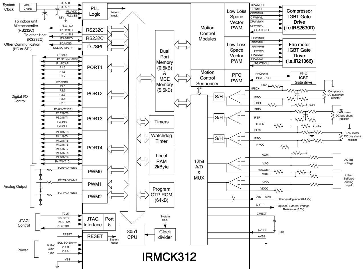
Figure 5. Application Connection of IRMCK312
