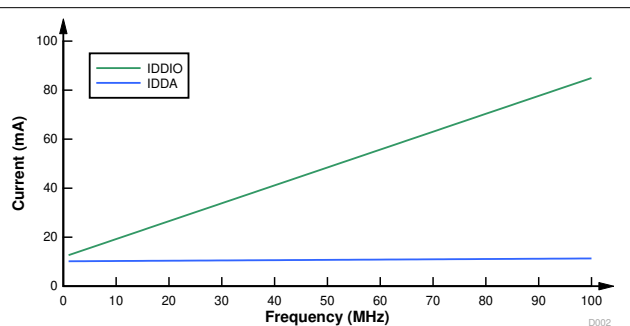
Figure 7-3. Current Versus Frequency — Internal VREG
