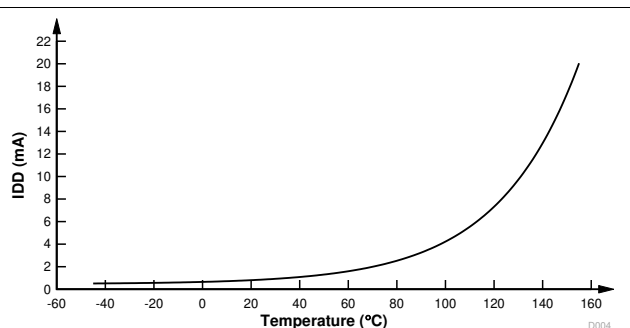
Figure 7-5. Halt Current Versus Temperature (°C)
