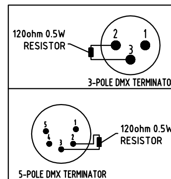
SCHEMATICS OF STANDARD DMX TERMINATOR
