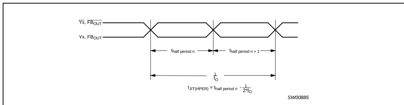
Figure 6. Half-period jitter
