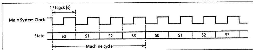
Figure 1-15. Machine cycle
