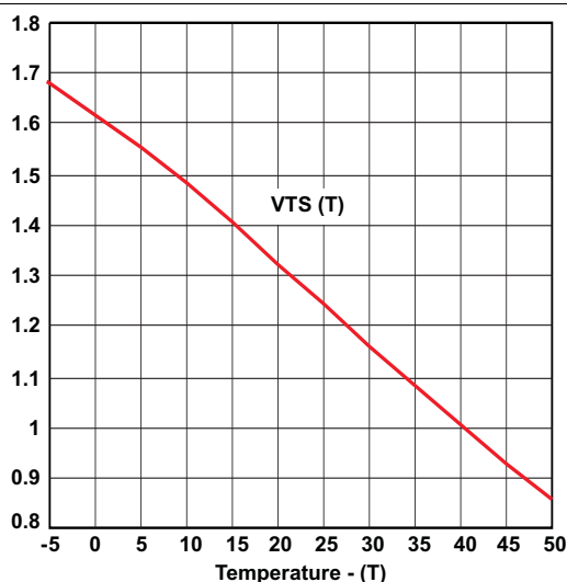
Figure 49. Resulting TS Voltage
