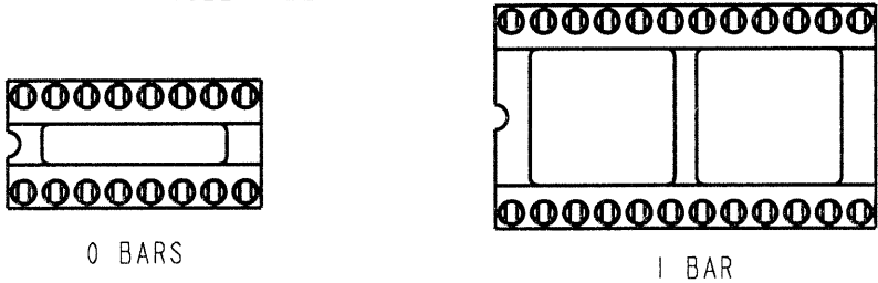
ILLUSTRATION OF NUMBER OF CENTRE BARS (SEE TABLE)
