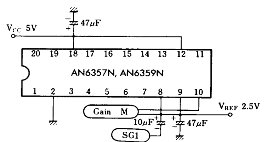
Test Circuit 9 (G V2 )
