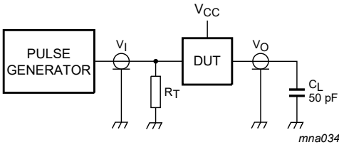
Test data is given in Table 8 . Definitions for test circuit: C_L = Load capacitance including jig and probe capacitance; R_T = Termination resistance should be equal to output impedance Z_o of the pulse generator. Fig. 5. Test circuit for measuring switching times
