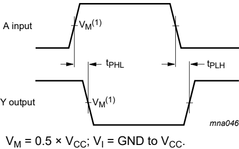
Fig. 4. The input (A) to output (Y) propagation delay times
