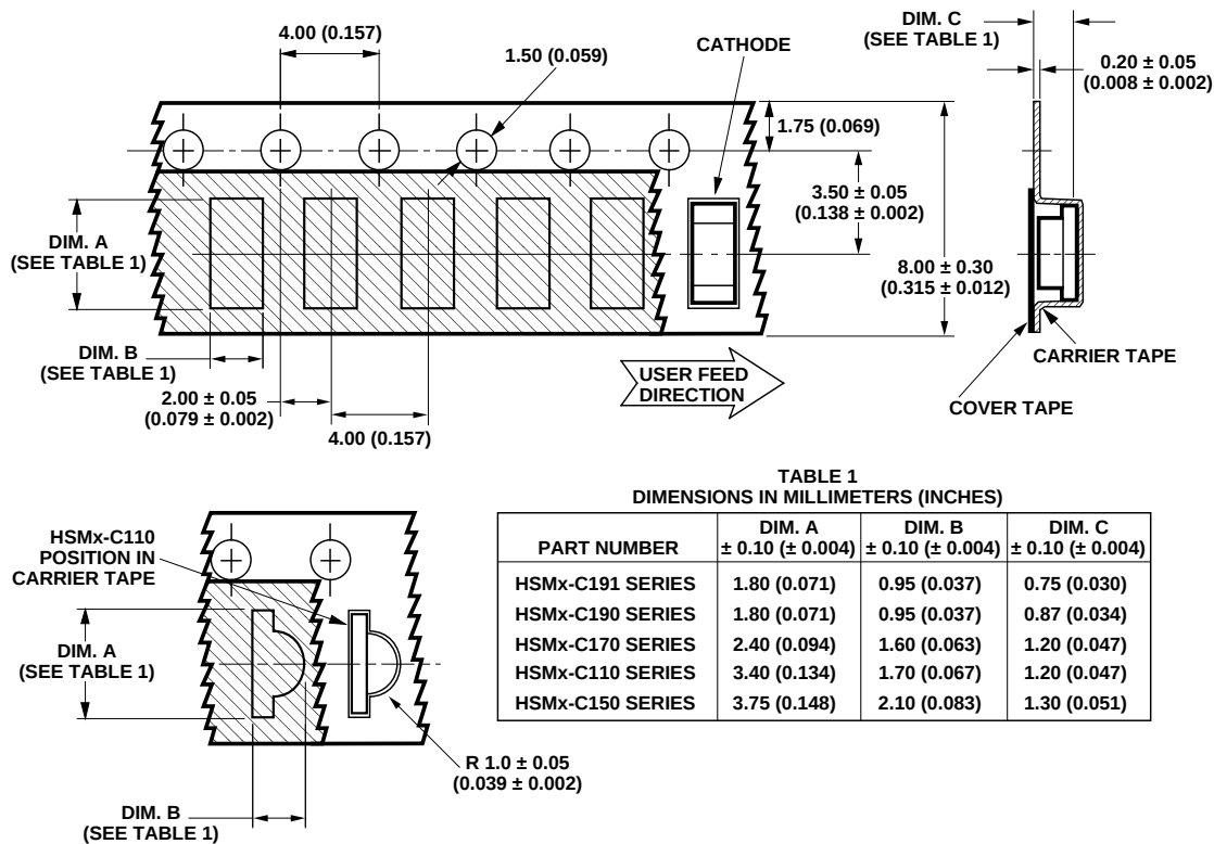
Figure 14. Tape dimensions.
