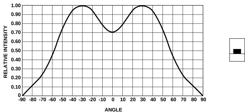
Figure 5. Relative intensity vs. angle for HSMx-C110.
