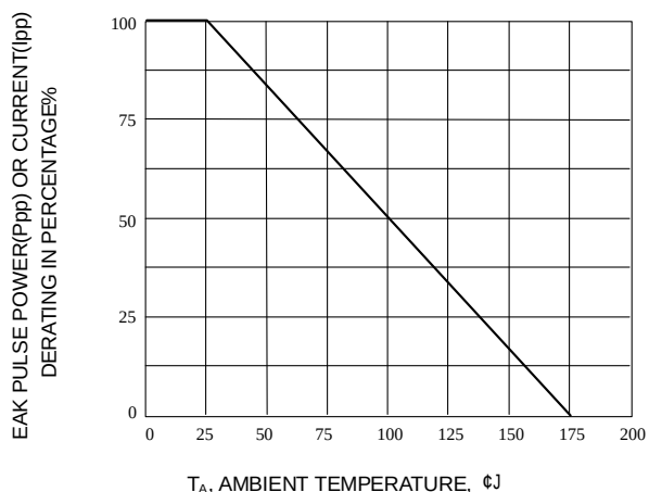
Fig. 2-PULSE DERATING CURVE
