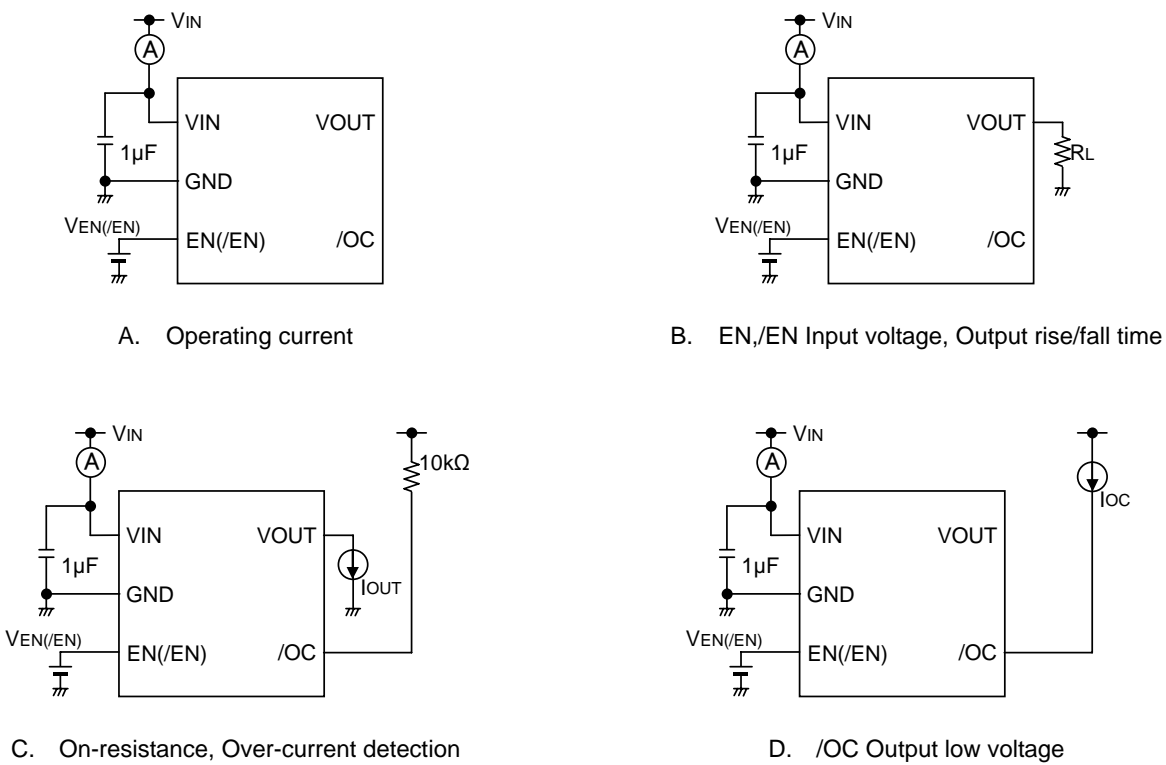
Figure 1. Measurement circuit
