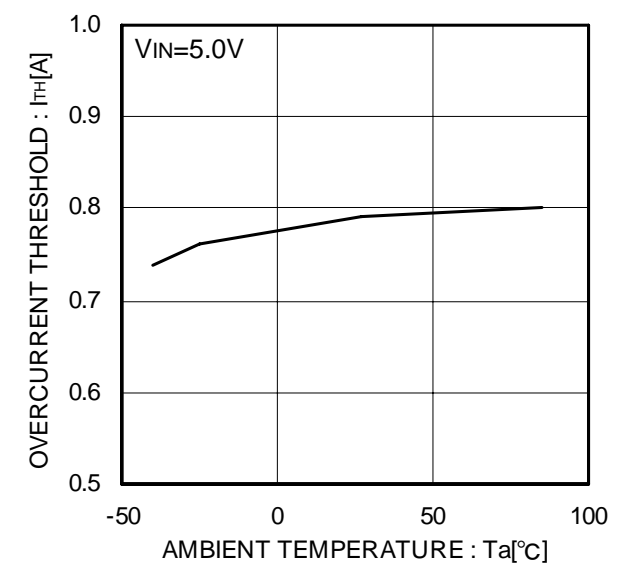
Figure 13. Over-current threshold
