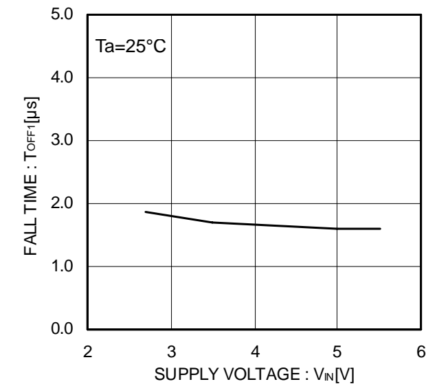
Figure 22. Output fall time
