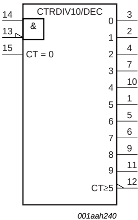
Fig 3. IEC logic symbol
