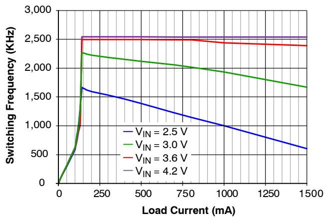
Figure 8. Frequency vs. Load Current and Input Voltage, Auto Mode, V_{OUT} = 1.8\text{ V} , Auto Mode
