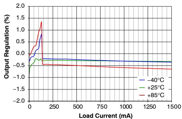
Figure 11. Output Regulation vs. Load Current and Temperature, V_{IN} = 3.6\text{ V} , V_{OUT} = 1.8\text{ V} , Auto Mode
