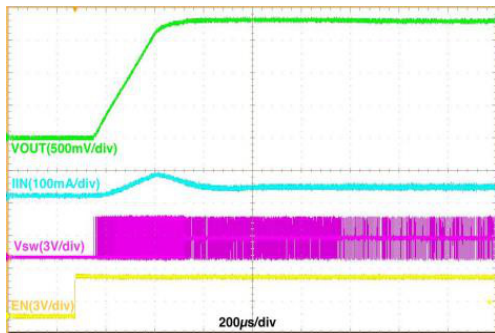
Figure 20. Start-up, V_{IN} = 3.6\text{ V} , V_{OUT} = 1.8\text{ V} , 50\text{ mA} Resistive Load, Auto Mode
