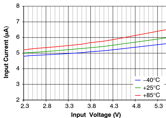
Figure 12. Quiescent Current vs. Input Voltage and Temperature, V_{OUT} = 1.8\text{ V} , Auto Mode
