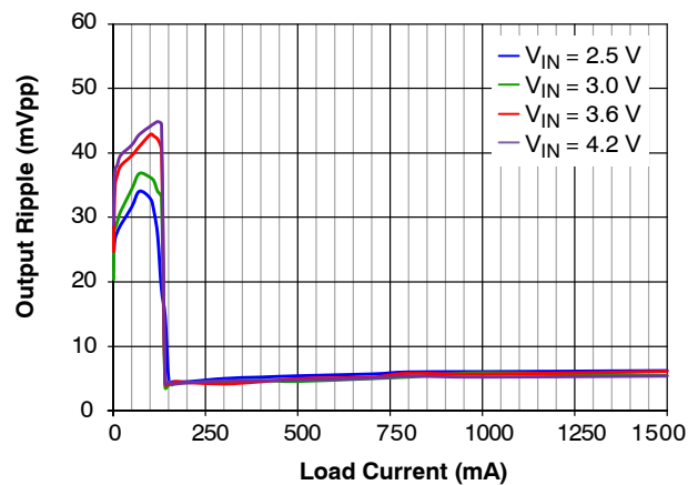
Figure 9. Output Ripple vs. Load Current and Input Voltage, V_{OUT} = 1.8\text{ V} , Auto Mode
