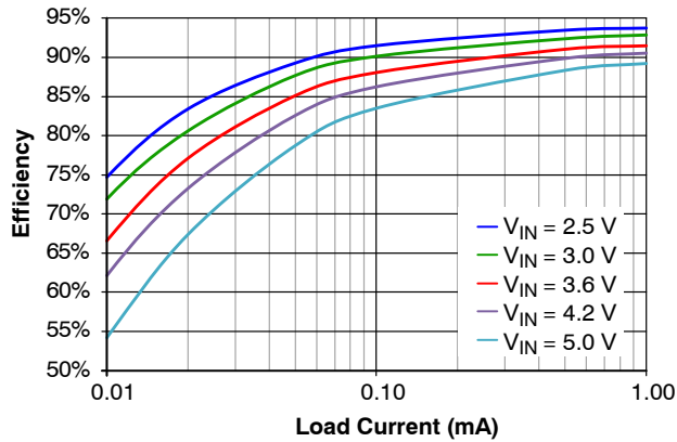
Figure 6. Efficiency vs. Load Current and Input Voltage, V_{OUT} = 1.8\text{ V} , SLIQ Mode
