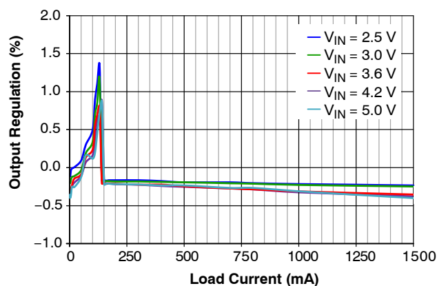
Figure 10. Output Regulation vs. Load Current and Input Voltage, V_{OUT} = 1.8\text{ V} , Auto Mode
