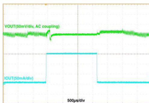
Figure 15. Load Transient, V_{IN} = 3.6\text{ V} , V_{OUT} = 1.8\text{ V} , 10 mA \leftrightarrow 150 mA, 1 \mu\text{s} Edge, Auto Mode
