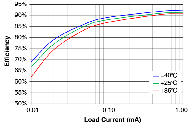
Figure 7. Efficiency vs. Load Current and Temperature, V_{IN} = 3.6\text{ V} , V_{OUT} = 1.8\text{ V} , SLIQ Mode
