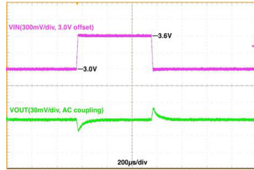
Figure 19. Line Transient, V_{IN} = 3.0\text{ V} \leftrightarrow 3.6\text{ V} , V_{OUT} = 1.8\text{ V} , 10\text{ }\mu\text{s} Edge, 300\text{ mA} Load, Auto Mode
