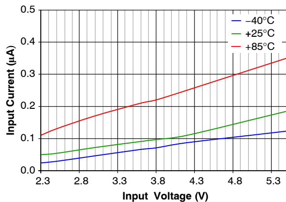
Figure 14. Shutdown Current vs. Input Voltage and Temperature
