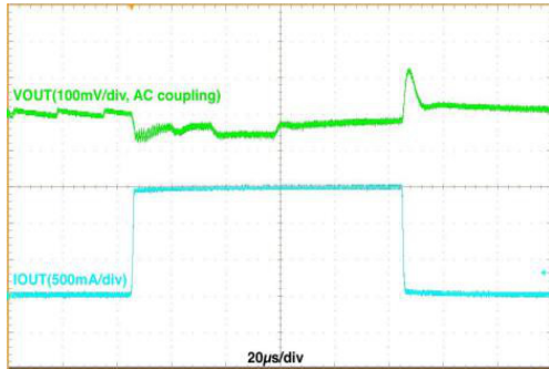
Figure 18. Load Transient, V_{IN} = 3.6\text{ V} , V_{OUT} = 1.8\text{ V} , 10\text{ mA} \leftrightarrow 1500\text{ mA} , 1\text{ }\mu\text{s} Edge, Auto Mode
