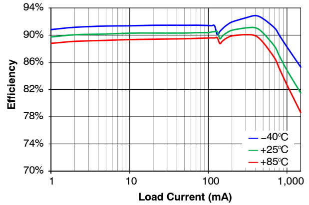
Figure 5. Efficiency vs. Load Current and Temperature, V_{IN} = 3.6\text{ V} , V_{OUT} = 1.8\text{ V} , Auto Mode
