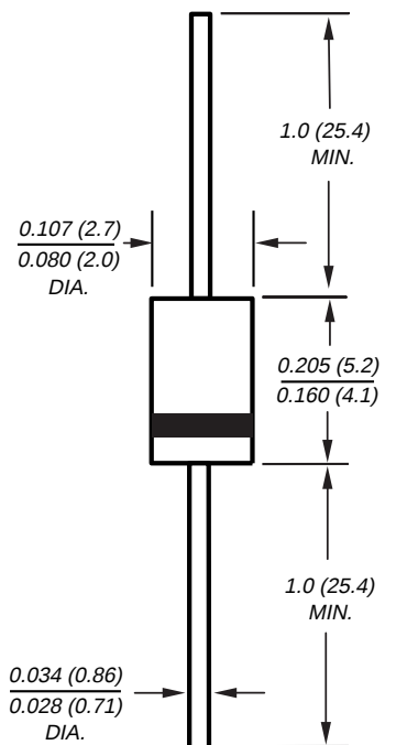
DO-204AL (DO-41 Plastic)
