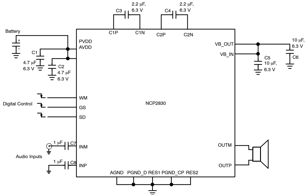
Figure 30. Single-Ended Configuration
