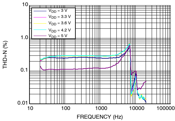
Figure 19. THD+N vs Frequency
