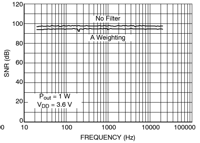
Figure 16. SNR vs Frequency
