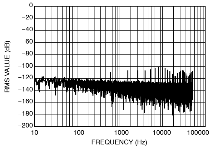
Figure 14. FFT of Switching Signal During GSM Burst
