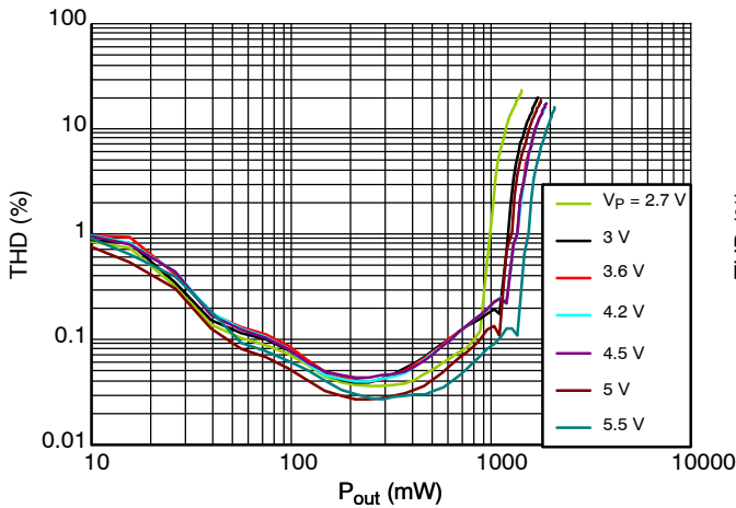
Figure 7. THD vs P_{out} R_L = 8 \Omega , WM = \text{Low}
