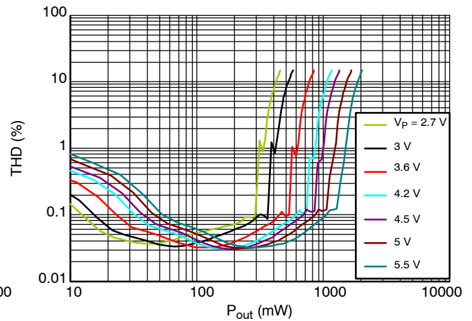
Figure 8. THD vs P_{out} R_L = 8 \Omega , WM = \text{High}
