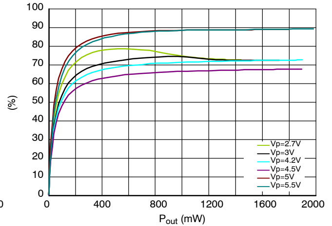
Figure 22. Global System Efficiency
