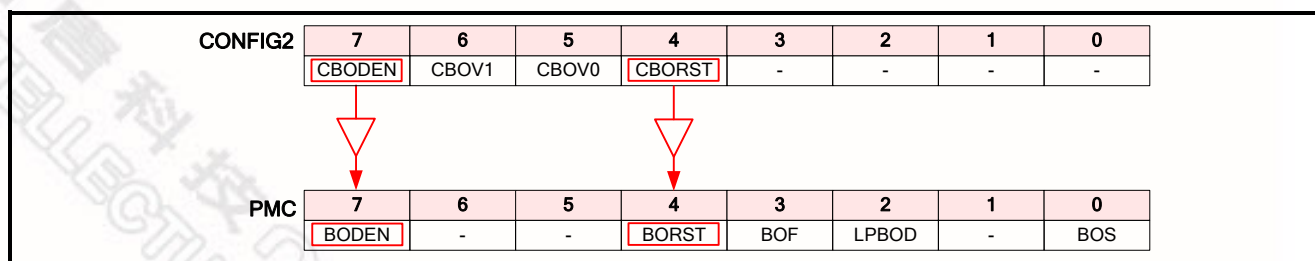
Figure 24–2. CONFIG2 Reset Reloading
