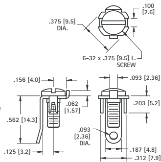
SOLDER TAB
