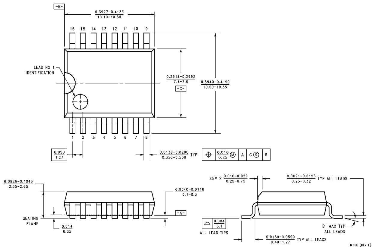
Figure 13. 16-Lead Small Outline Integrated Circuit (SOIC), JEDEC MS-013, 0.300" Wide Package Number M16B
