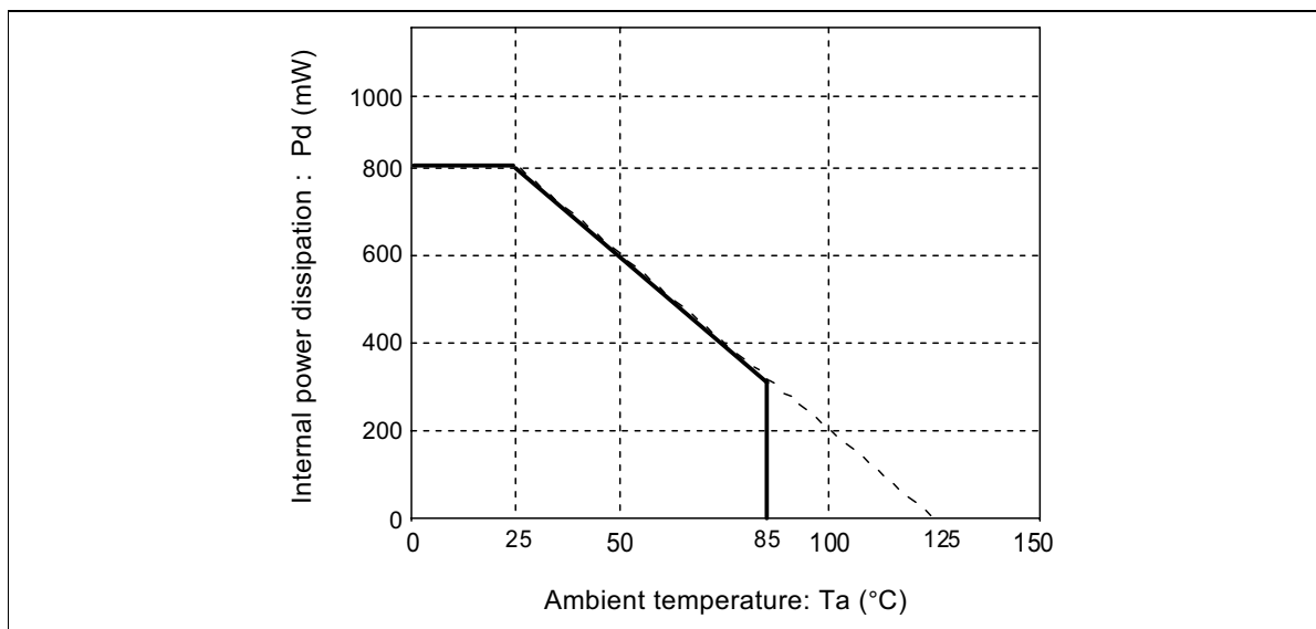
Figure 1 Thermal derating curve
