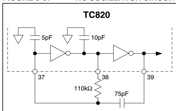
FIGURE 5-5: RC OSCILLATOR CIRCUIT
