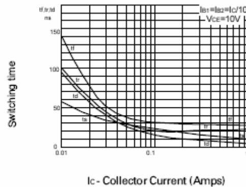
Switching Speeds
