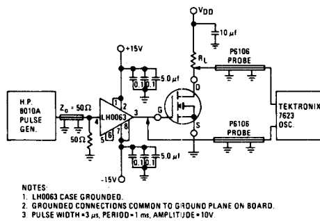
Fig. 15 - Switching Time Test Circuit
