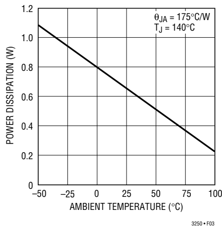
Figure 3. Maximum Power Dissipation vs Ambient Temperature
