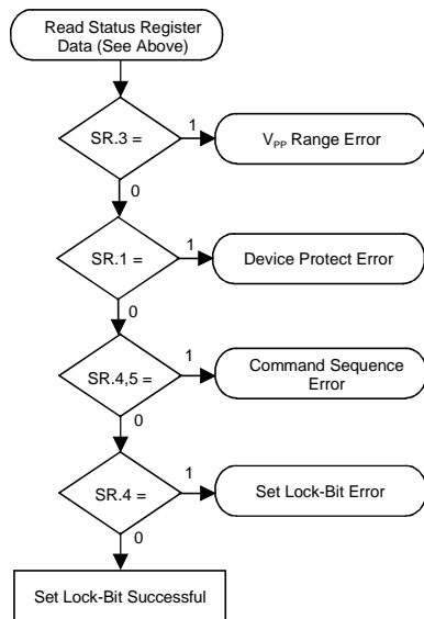
Figure 10. Set Block and Master Lock-Bit Flowchart
