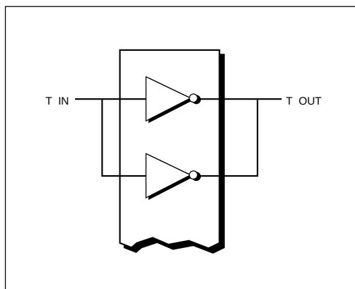
Figure 5. Parallel Drivers
