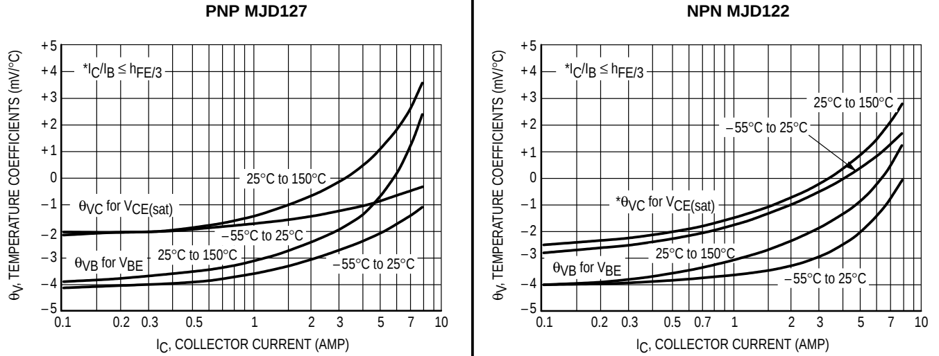
Figure 5. Temperature Coefficients
