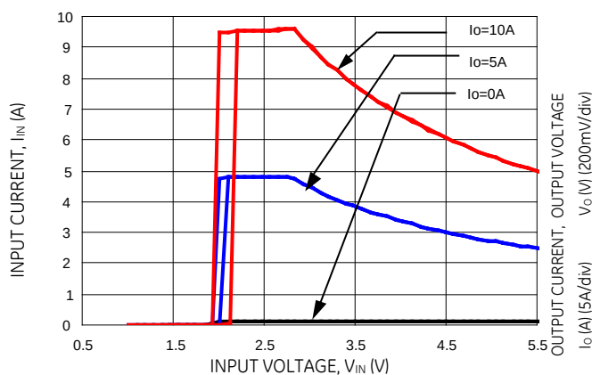
Figure 7. Input voltage vs. Input Current ( V_O = 2.5Vdc ).
