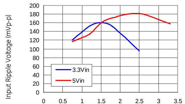
Figure 27. Input ripple voltage for various output with 1 \times 150\mu F polymer and 1 \times 47\mu F ceramic capacitors at the input (full load).
