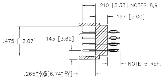
SECTION H-H
