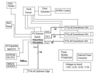
89KTPES32H8G2 Evaluation Board Functional Diagram
