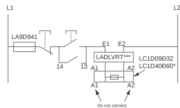
Typical Wiring Scheme for 3-Wire Control
