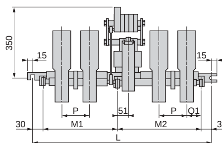
4-pole contactors
