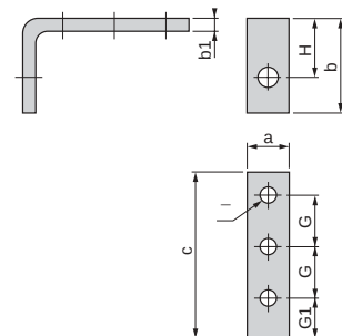
Wide range brackets LA9F•980 (set of 3)
