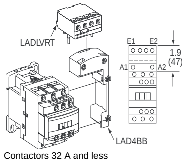
Contactors 32 A and less
