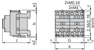
LC2D09 to D38 2 x LC1D09 to D38
