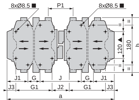
Reversing contactors 2 x CR1F400 to CR1F630
