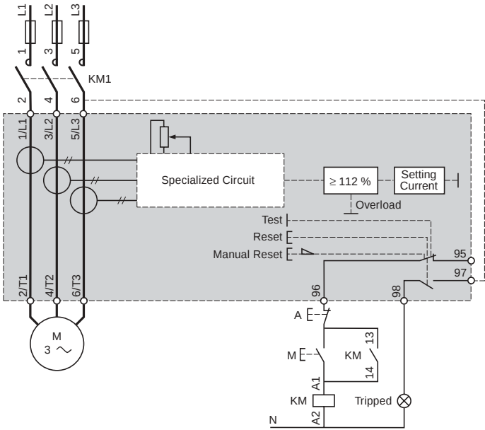
Wiring Diagram LR9F
