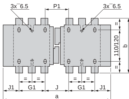
Reversing contactors 2 x CR1F150 to CR1F265 Horizontally mounted
